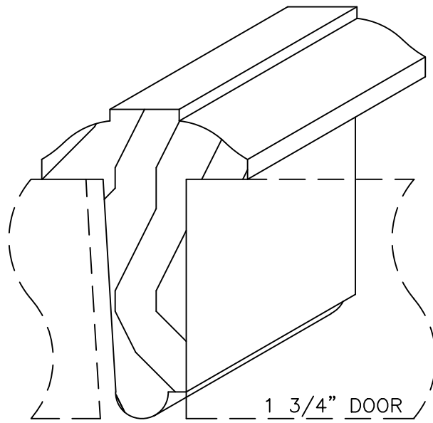
OPERABLE INTERIOR ASTRAGAL
