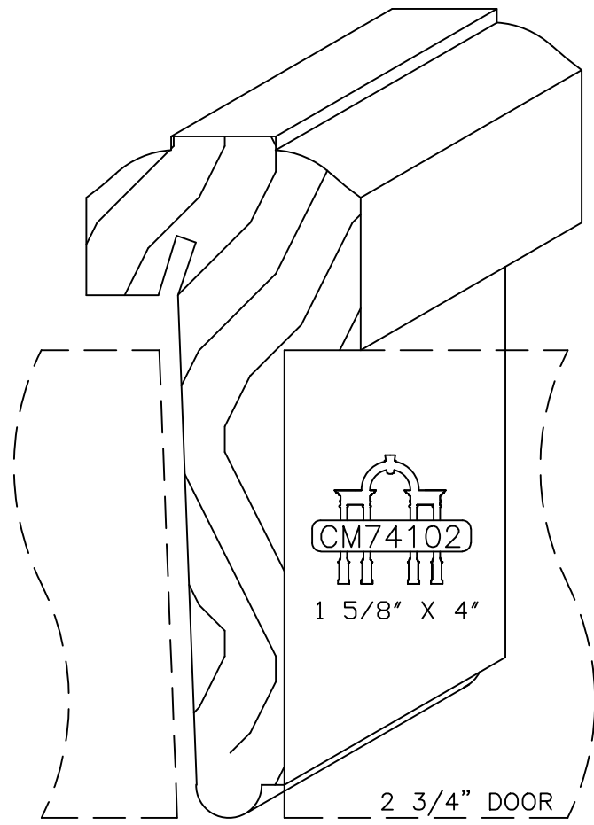
OPERABLE EXTERIOR ASTRAGAL
