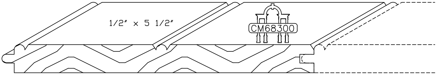
DOUBLE BEADED V-JOINT T&G
