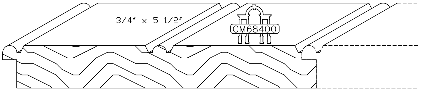
DOUBLE BEADED V-JOINT T&G
